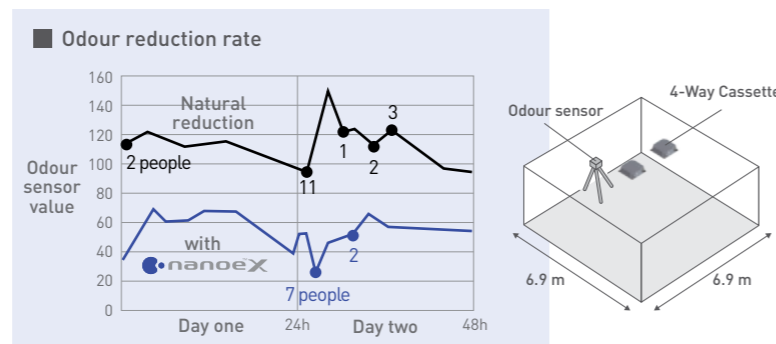
Tested Product: CS-P45U4B (4-way ceiling cassette type equipped with nanoe™ X) x 2 units Evaluation: October 8, 2019, to October 17, 2019 (1) Tested using the units installed in an approximately 47m² conference room Gunma Factory in Japan. (2) Air conditioner settings Operation mode: Air conditioning, Preset temperature: 27°C, Wind direction: Horizontal, Wind speed: Medium wind speed (3) During the first week, the nanoe™ X was operated, and during the second week, the nanoe™ X was stopped and the air conditioner was operated, and the odour intensity was measured for two days each with the New Cosmos Electric odour sensor (XP-329m) (4) The air conditioner was operated for 24 hours and tested. Target odour: Room odour
