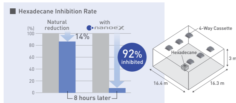
Tested Product: 4-Way Cassette x 6 units, Area: Approx. 802m³ [Approx. 16.4m x 16.3m x 3m], Hazardous Substance: Hexadecane*2, Test Conditions: 8-hour exposure with 4-Way Cassette (Fan mode and nanoe™ X functionality), Test Result: nanoe™ X turned ON=hexadecane inhibition avg. 92%, nanoe™ X turned OFF=hexadecane inhibition avg. 14%
